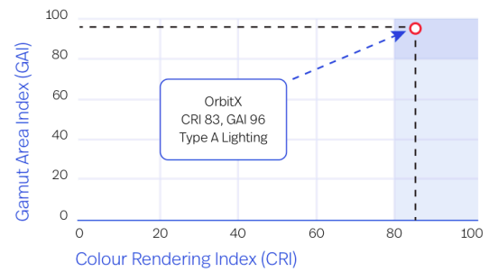
Type A Lighting*
